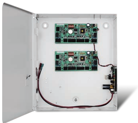
URC-2004... includes two URC-2000 controllers, enclosure, and power supply
