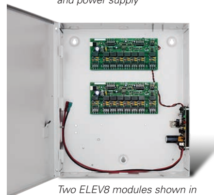
Two ELEV8 modules shown in enclosure with power supply
